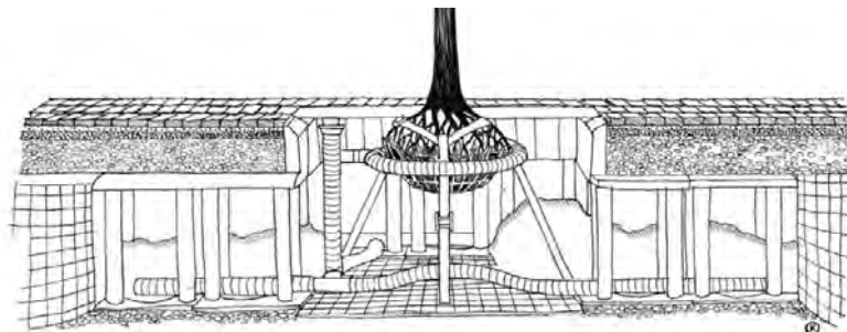
Figure 26: Example of installed soil cells system around a newly planted tree.
